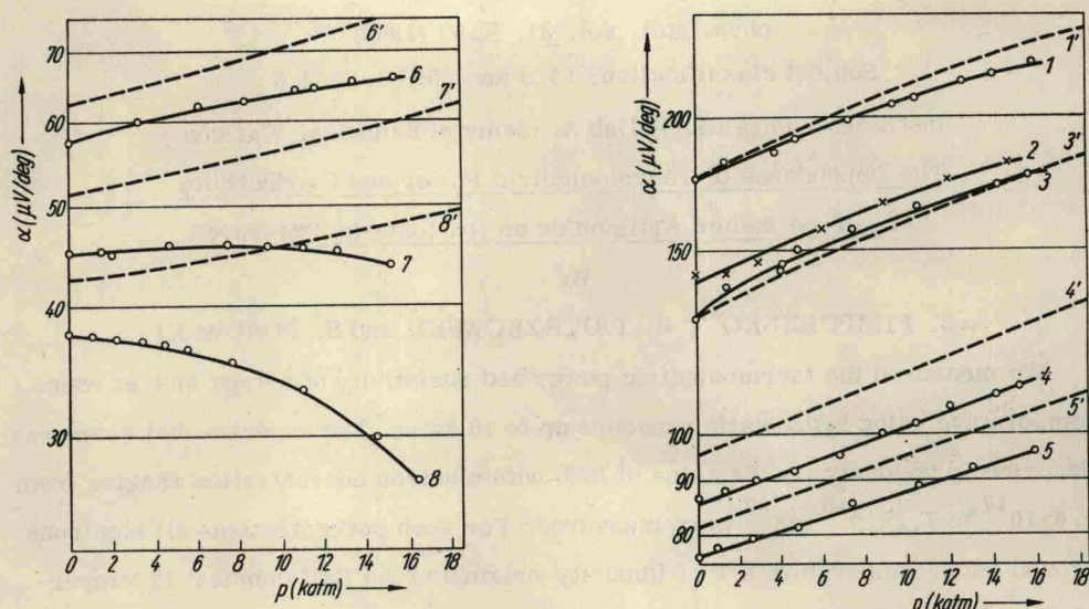
Fig. 1. Dependence of thermoelectric power on pressure; solid curves - experiment, dashed curves - theoretical, electron concentration:
